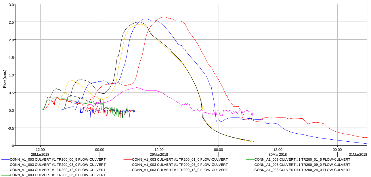
Figura 6-6 – Idrogrammi Tr 200 CONN_A1_003_C1
